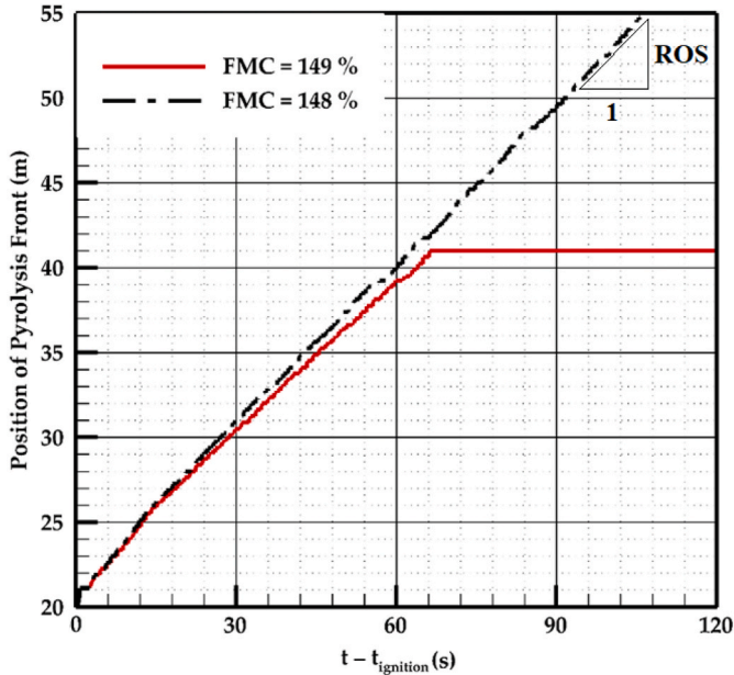
Fig. 2. Time evolution of the pyrolysis front position obtained under marginal conditions for U_{10} = 4 m/s and e = 0.5 m ( \delta = 0.5 kg/m 2 ). The ROS is the curve slope obtained at steady fire spread.
