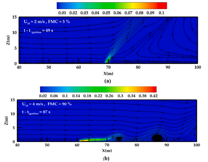
Fig. 12. Distribution of water-vapour mass-fraction and flow streamlines obtained (a) for U_{10} = 2 \text{ m}/\text{s} , \text{FMC} = 5\% , and e = 0.5 \text{ m} , and (b) for U_{10} = 4 \text{ m}/\text{s} , \text{FMC} = 90\% , and e = 0.5 \text{ m} .
