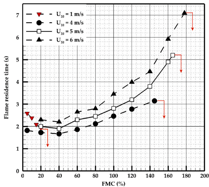
Fig. 10. Fire residence time versus the FMC, obtained for a fuel-bed thickness e = 0.5 \text{ m} ( W = 0.5 \text{ kg}/\text{m}^2 ) and for different wind speeds. The vertical arrow indicates the FMC threshold of extinction.
