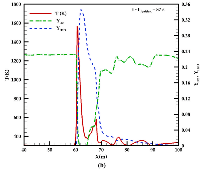
Fig. 6. Profiles of the gas temperature and the mass fraction oxygen and water vapour in the gas mixture, obtained at the surface of the vegetation cover ( z = e ) for e = 0.5 m ( W = 0.5 kg/m 2 ), for U_{10} = 4 m/s, and for two values of FMC: (a) FMC = 5%, (b) FMC = 90%.
