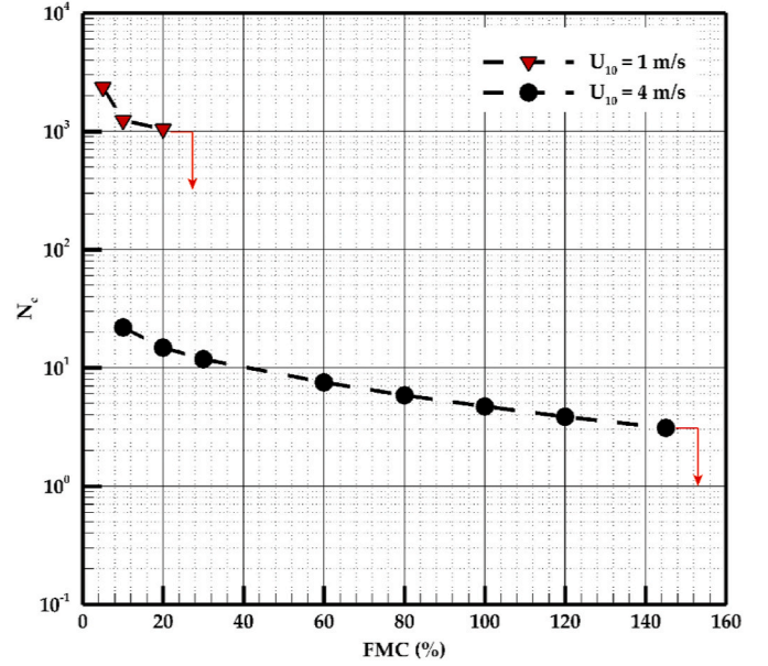
Fig. 11. Byram's convective number versus the FMC, obtained for a fuel-bed thickness e = 0.5 \text{ m} ( W = 0.5 \text{ kg}/\text{m}^2 ) and for U_{10} = 1 and 4 \text{ m}/\text{s} . The vertical arrow indicates the FMC threshold of extinction.
