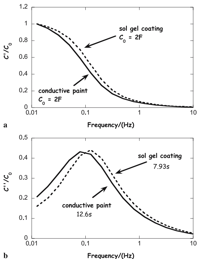
FIGURE 9 Evolution of the real part (a) and imaginary part (b) of capacitance vs. frequency for 2.3 \text{ V}-2 \text{ F} supercapacitor laboratory cell
