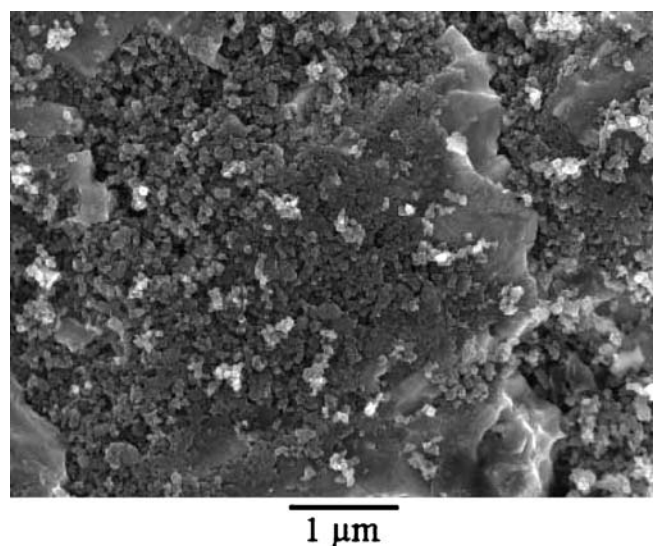
FIGURE 2 FEG-SEM picture of an etched Al current collector, covered by a carbonaceous coating by the sol-gel route
