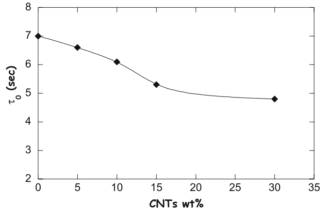
FIGURE 11 Variation of relaxation time constant with CNTs content
