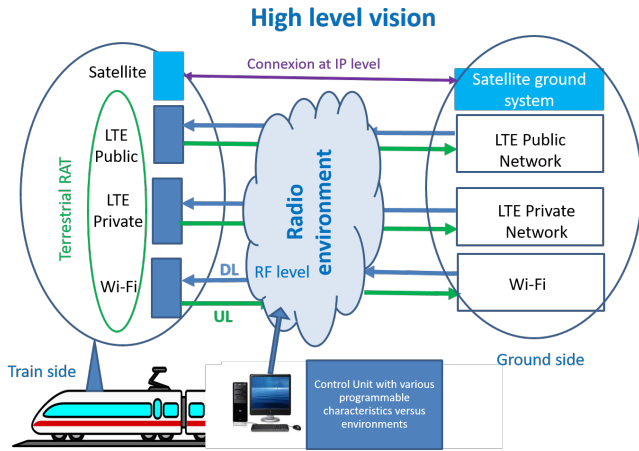
FIGURE 2. High level vision of the Emuradio4Rail platform
