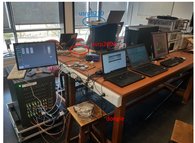
FIGURE 5. The Emuradio4Rail platforms with one Wi-Fi and two LTE bearers emulated by OAI
