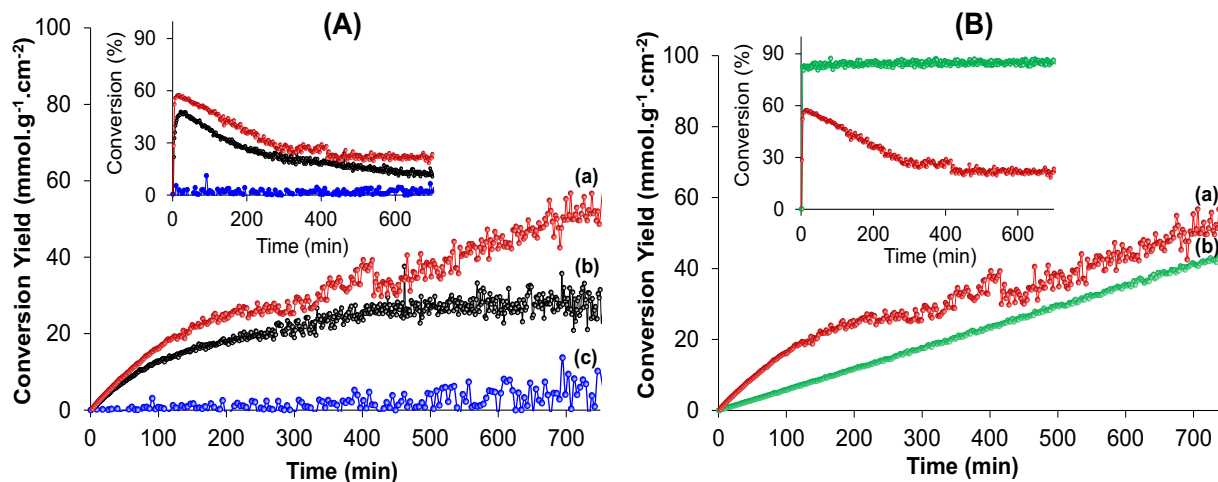
Figure 1. (A) Effect of the activation temperature on the photocatalytic activity of Ag/ZX-Bi (a) activated at 200 °C (Ag/ZX-Bi_200), (b) activated at 120 °C (Ag/ZX-Bi_120) and (c) non-activated (Ag/ZX-Bi_NA). (B) Effect of the MeOH initial concentration (a) 10350 ppm and (b) 2100 ppm on the photocatalytic activity of Ag/ZX-Bi_200. The insert corresponds to the methanol conversion in % as a function of reaction time. Reaction condition: [MeOH]=10350 (~1%) for A in 20%O 2 /Ar; m catalyst =20mg; Lampe Xe with filter pass high ( \lambda > 390\text{nm} ); irradiance = 71 mW/cm 2 ; Total flow= 25 cm 3 /min. Catalysts activated at 120 or 200 °C under Ar for 30 min in dark followed by 30 min under visible irradiation; heating rate = 2°C/min.
