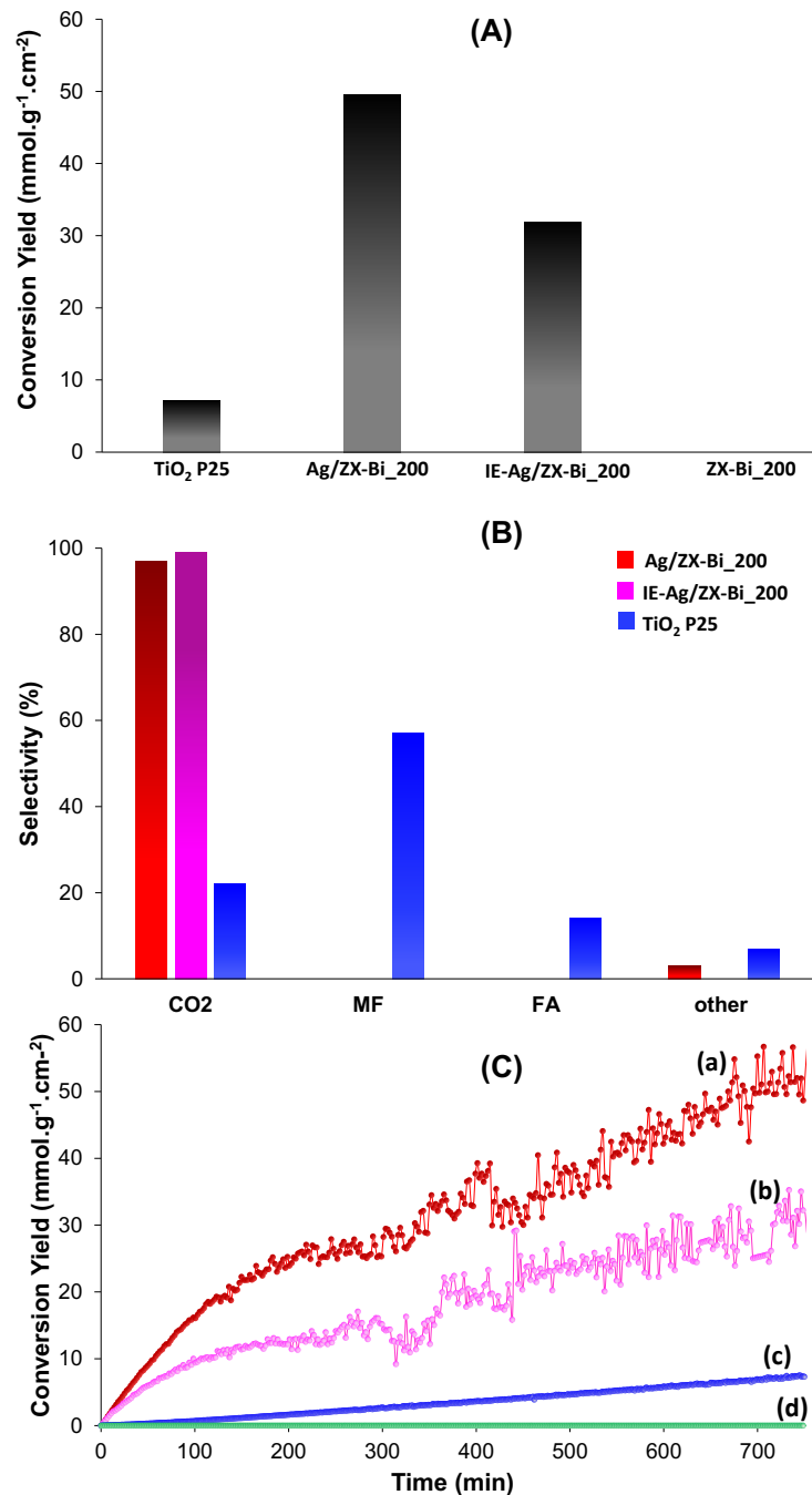
Figure 2. (A) Methanol conversion yield (in mmol per gram of catalyst per cm 2 of irradiated surface) and (B) selectivity (%) calculated at t = 720 min (~12h) of reaction and (C) evolution of the methanol conversion versus the irradiation time on (a) Ag/ZX-Bi_200, (b) IE-Ag/ZX-Bi_200, (c) TiO 2 P25 and (d) ZX-Bi_200 samples. Reaction conditions: [MeOH]= 10350 ppm in 20%O 2 /Ar; m catalyst =20mg; Lampe Xe with filter pass high ( \lambda > 390\text{nm} ); irradiance = 71 mW/cm 2 ; Total flow= 25 cm 3 /min. Catalysts activated at 200 °C under Ar for 30 min in dark followed by 30 min under visible irradiation; heating rate = 2°C/min.
