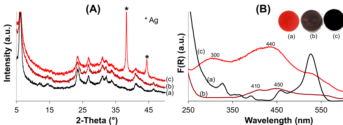
Figure 4. (A) X-ray diffractograms and (B) DR-UV-visible spectra of Ag/ZX-Bi: (a) as-prepared, (b) after activation at 200 °C under Ar and (c) then 12 h of the photocatalytic test. Reaction conditions: [MeOH]= 10350 ppm in 20%O 2 /Ar; m_{\text{catalyst}}=20\text{mg} ; Lampe Xe with filter pass high ( \lambda>390\text{nm} ); irradiance = 71 mW/cm 2 ; Total flow= 25 cm 3 /min. Catalysts activated at 200 °C under Ar for 30 min in dark followed by 30 min under visible irradiation; heating rate = 2°C/min.
