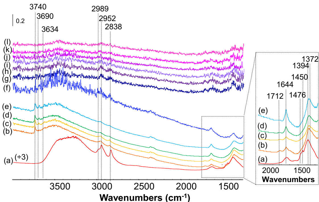
Figure 3. Evolution of the IR spectra of Ag@ZX-Bi 200 during the photooxidation of methanol during the first minutes of irradiation: (a) 0, (b) 2, (c) 4, (d) 6, (e) 10 min and at prolonged time (f) 2, (g) 4, (h) 6, (i) 8, (j) 10, (k) 11 and (l) 12 h of visible light irradiation at 25 °C. on the right: zoom on the 1500-2000 cm -1 region of the catalyst surface in the first minutes of irradiation. reaction condition: MeOH=10350 ppm; 20%O 2 /Ar; Lamp Xe ( \lambda > 390 nm); irradiance = 71 mW/cm 2 ; total flow=25 cm 3 /min; m cat =20 mg.
