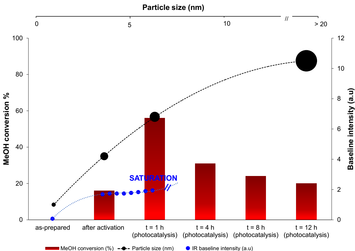
Figure 6. Correlation of MeOH conversion % with the particle size (nm) and the baseline intensity of the IR surface of Ag@ZX-Bi_NA and Ag@ZX-Bi_200 and of Ag@ZX-Bi_200 after various time of the photocatalytic tests under visible irradiation at RT. The as-prepared (Ag@ZX-Bi_NA) sample is added for comparison.
