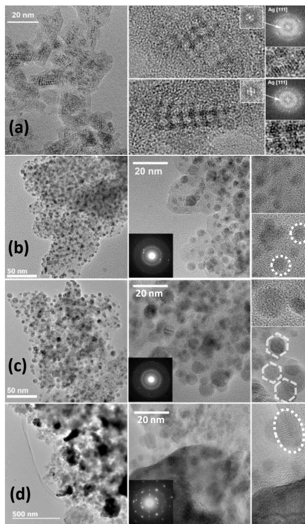
Figure 5. TEM images of: (a) the as-prepared Ag/ZX-Bi catalyst, (b) after activation at 200 °C under Argon, and of Ag@ZX-Bi_200 after (c) 1 and (d) 12 h of the photocatalytic tests. Reaction conditions: [MeOH]= 10350 ppm in 20%O 2 /Ar; m catalyst =20mg; Lampe Xe with filter pass high ( \lambda > 390\text{nm} ); irradiance = 71 mW/cm 2 ; Total flow= 25 cm 3 /min. Catalysts activated at 200 °C under Ar for 30 min in dark followed by 30 min under visible irradiation; heating rate = 2°C/min.
