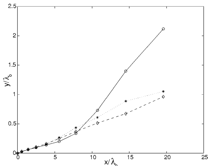
FIG. 11. Streamwise evolution of the lateral dispersion. (○) Case A; (*) case B; (◇) case C.
