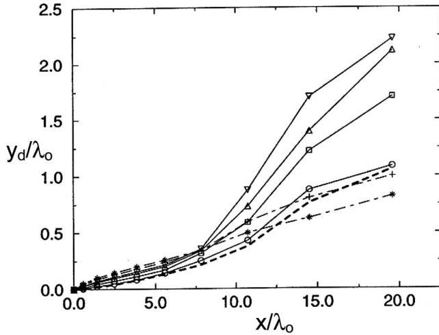
FIG. 3. Lateral dispersion of bubbles of various sizes in the mixing layer. (Dashed line) Fluid particle; (O) \delta=2.77 \times 10^{-4} ; (□) \delta=5.55 \times 10^{-4} ; (△) \delta=6.94 \times 10^{-4} ; (▽) \delta=7.63 \times 10^{-4} ; (+) \delta=9.02 \times 10^{-4} ; (*) \delta=10.4 \times 10^{-4} .
