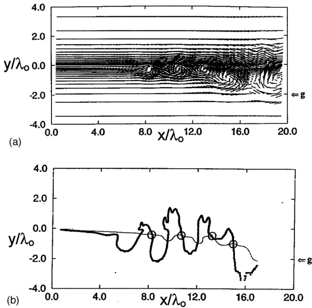
FIG. 1. Snapshot of the single-phase mixing layer. (a) Velocity field \mathbf{u} - U_m \mathbf{e}_x . (b) (○) Position of the stable fixed points ( \delta = 6.94 \times 10^{-4} , Fr = 40 ). Bold line ( f_x(x,y)=0 ); thin line ( f_y(x,y)=0 ).
