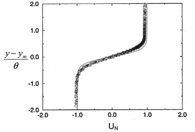
FIG. 8. Profiles of the normalized streamwise velocity U_N=(U(x,y) - U_m(x))/\Delta U(x) vs the dimensionless lateral position (y - y_m(x))/\theta(x) . Symbols correspond to distinct streamwise locations. (Solid line) tanh profile.
