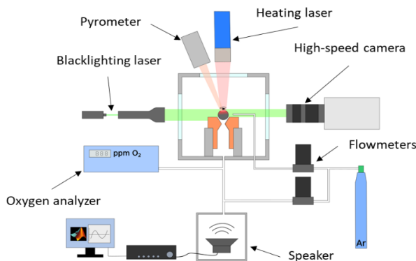
66 67 Fig. 3. Scheme of levitation device.
