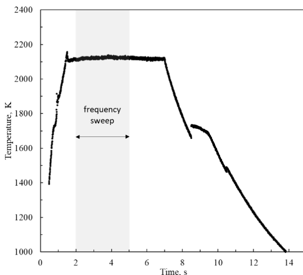
Fig. 2. Standard temperature measurement on a sample.
