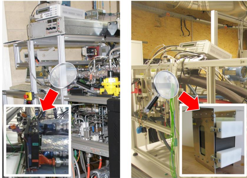
Fig. 1. Pictures of the two investigated PEMFCs and testbenches. Left: CEA LITEN stack. Right: RBZ - Inhouse Engineering GmbH stack.
