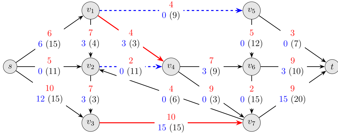
FIG. 1 – Example of a Maximum Flow Blocker Problem with a target flow value F = 23 .
