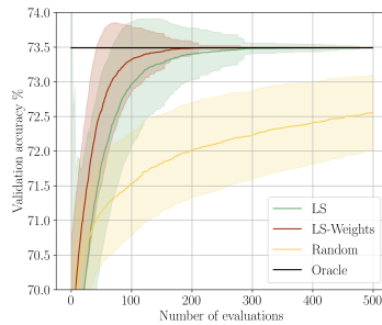
(b) Cifar100
