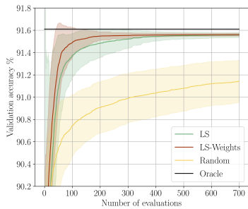
(a) Cifar10
