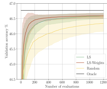
(c) ImageNet16-120
