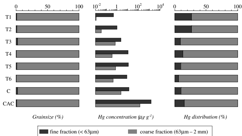
Fig. 5. Percentages of fine and coarse fractions, total mercury concentrations and abundance of mercury in each fraction for the different sampling station of the Thur River basin. CAC represents bottom sediments collected in the chlor-alkali channel.
