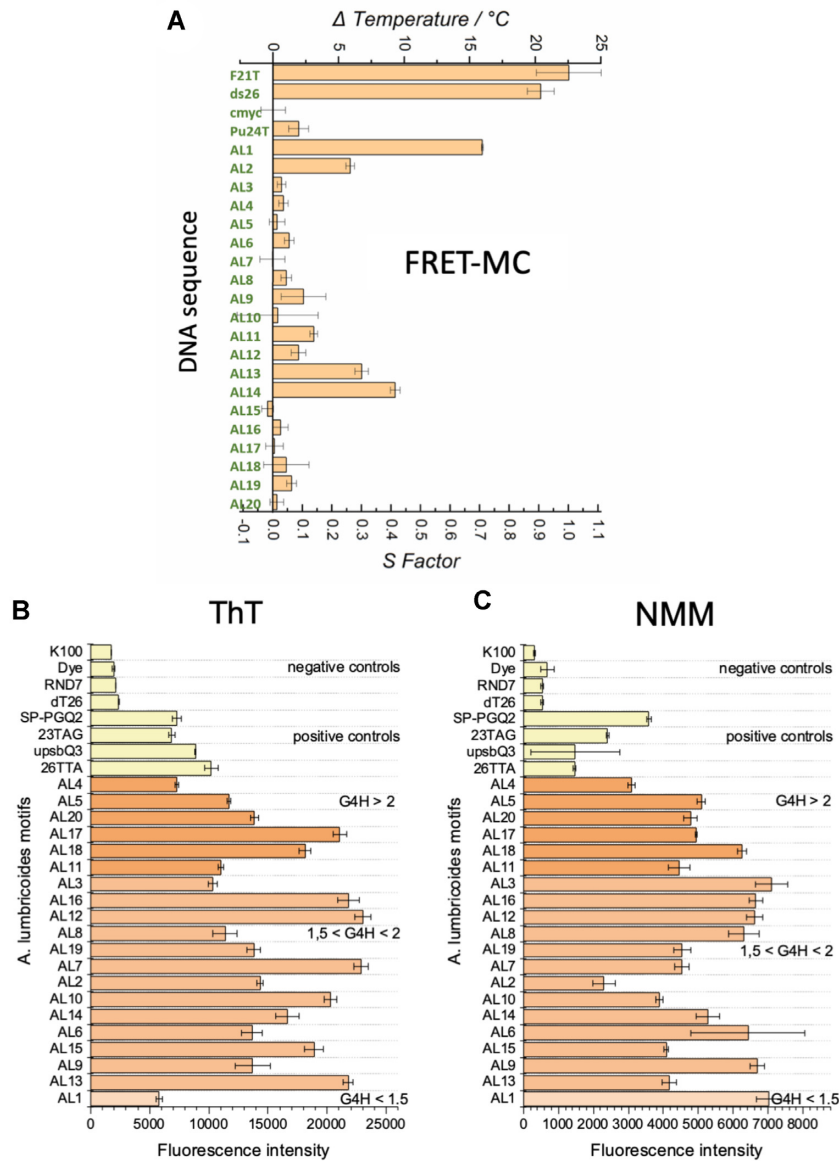
Figure 5. Evidence for G-quadruplex formation with 20 Ascaris lumbricoides sequences. (A) FRET MC results. (B) Thioflavin T fluorescence emission and (C) NMM fluorescence emission. Both Thioflavin T and NMM are light-up probes for which fluorescence intensity increases in the presence of G4-forming sequences.
