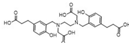
HBED-CC (log K_{\text{GaL}} = 38.5) [66]
