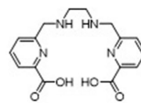
H 2 DEDPA (log K_{\text{GaL}} = 28.1) [66]
