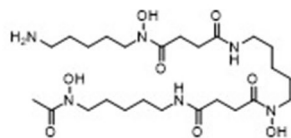
DFO (log K_{\text{GaL}} = 28.7) [66]
