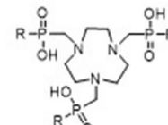
TRAP-H: R = H (log K_{\text{GaL}} = 21.9) TRAP-Pr: R = CH 2 CH 2 COOH (log K_{\text{GaL}} = 26.2) [85]
