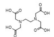
EDTA (log K_{\text{GaL}} = 21.7) [218]
