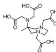
AAZTA (log K_{\text{GaL}} = 22.2) [66]
