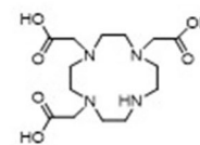
DO3A (log K_{\text{GaL}} = 24.6) [65]
