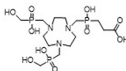
NOPO (log K_{\text{GaL}} = 25) [66]
