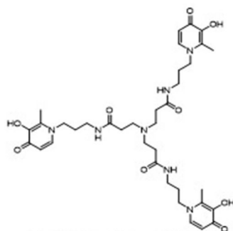
NTP(PrHP) 3 (log K_{\text{GaL}} = 33.3) [73]
