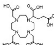
DOTAGA (log K_{\text{GaL}} = 21.3) [66]
