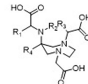
DATA M (log K_{\text{GaL}} = 21.5) [66]
