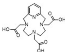
PCTA (log K_{\text{GaL}} = 19.4) [218]
