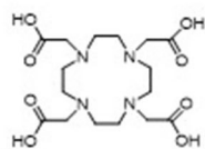
DOTA (log K_{\text{GaL}} = 21.3) [66]
