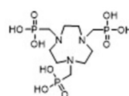
NOTP (log K_{\text{GaL}} = /) [86]
