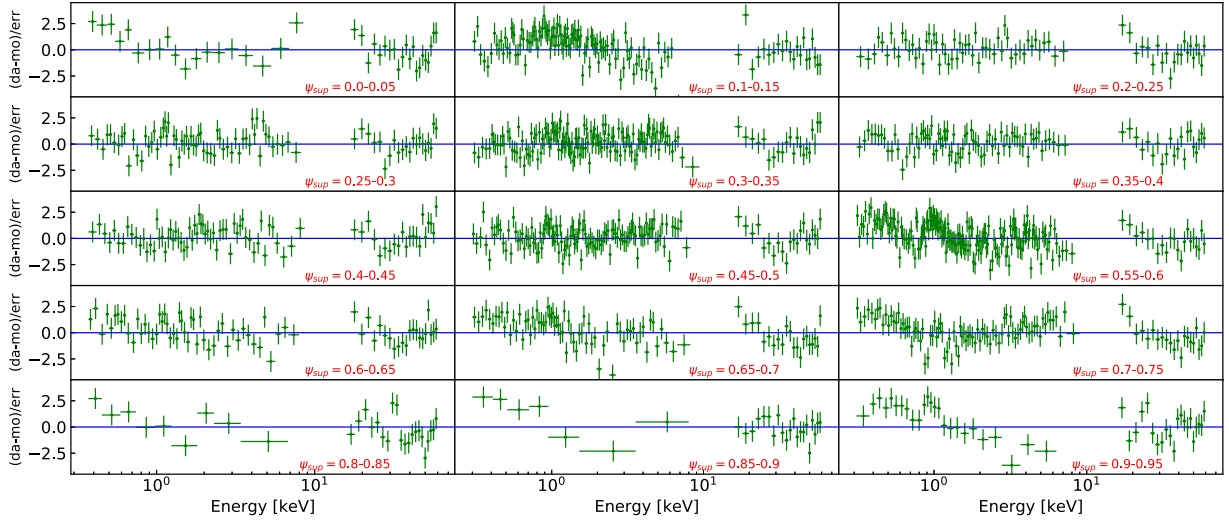
Figure 12. Residuals, for each XRT + BAT superorbital phase-resolved spectra, of the fit with the model \text{CONST*TBABS*K}_2(\text{DISKBB} + \text{COPLREFL} + \text{BW}) .
