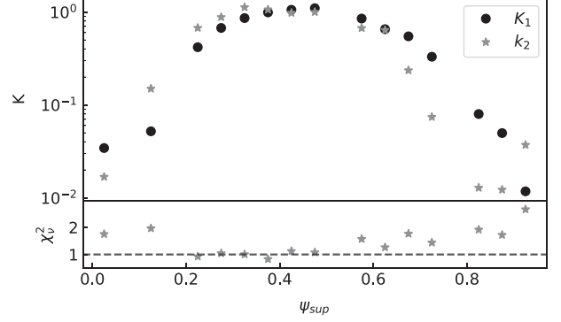
Figure 11. Upper panel: comparison of the coefficients K_1 (black points) and K_2 (grey stars); the magnitudes of the error bars are contained in the size of the data points. Lower panel: \chi^2_v resulting from the fit of the superorbital phase-resolved broad-band (XRT + BAT) spectra with the model \text{CONST} * \text{TBABS} * K_2 * (\text{DISKBB} + \text{COPLREFL} + \text{BW}) , where all the model parameters are fixed, while the K_2 term and the CONST term for the BAT data are the only free parameters.
