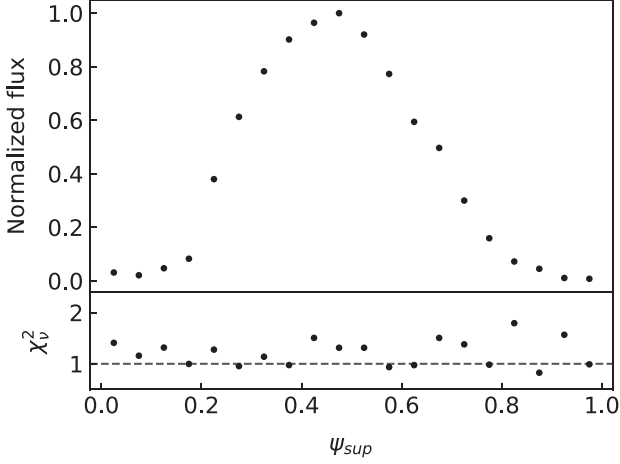
Figure 10. Upper panel: flux variation along the different superorbital phases with respect to the maximum. Lower panel: \chi^2_v resulting from the fit of the superorbital phase-resolved BAT spectra with the model K_1 * (\text{COPLREFL} + \text{BW}) , where all the model parameters are fixed, while the K_1 term is the only free parameter.
