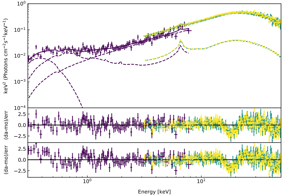
Figure 7. Best fit of the high-flux data with the phenomenological model \text{CONST*TBABS*(DISKBB + COPLREFL + HIGHECUT*POW)} (upper panel) and its residuals (middle panel). Swift /XRT, NuSTAR A, and NuSTAR B data are represented in violet, azure, and yellow, respectively (from dark to lighter colours for a grey-scale visualization). Lower panel: the residuals obtained without the soft blackbody component provide evidence that an additional component is needed to flatten the soft excess at lower energies.
