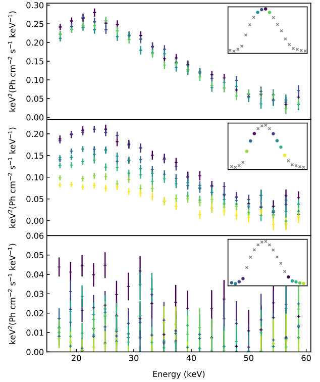
Figure 4. BAT superorbital resolved spectra unfolded through a power-law model with photon index = 0 . Spectra have been divided into three groups, depending on their flux level, for easy visual inspection. The colour code refers to the superorbital phase to which the spectra belong, which is shown in the inset of each panel.
