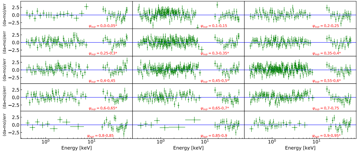
Figure 13. Residuals, for each XRT + BAT superorbital phase-resolved spectra, of the fit with the model \text{CONST*TBABS*}(\text{DISKBB} + \text{COPLREFL} + \text{K}_1\text{*BW}) . We marked with an asterisk (*) those phases for which we added an additional Gaussian component at \sim 1 keV to flatten the residuals and improve the statistic (see text for details).
