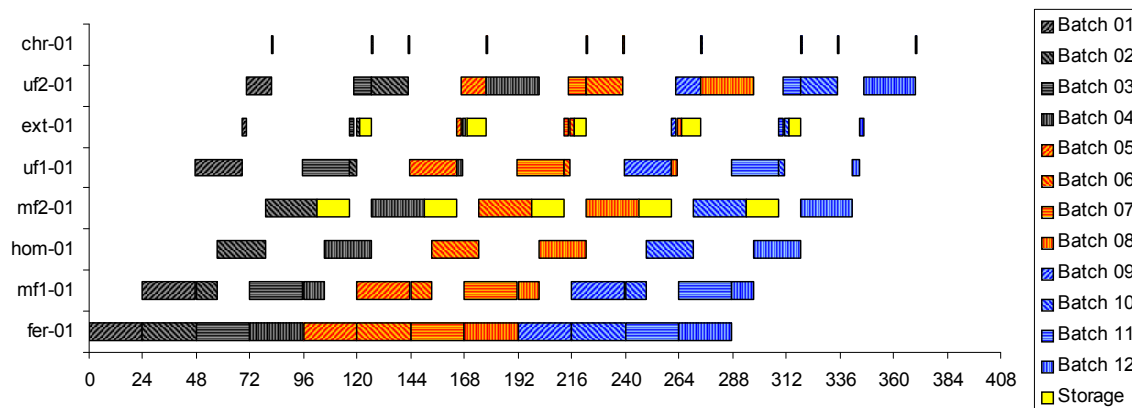
Figure 6. Simulation results for the multiproduct campaign policy
