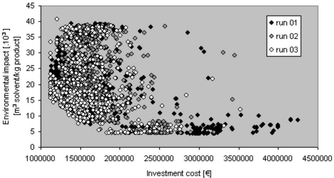
Figure 15. Pareto's optimal solutions Cost – Solvent (different optimization runs)
