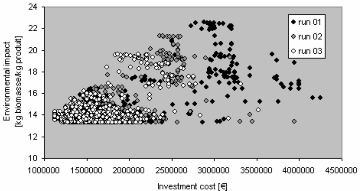
Figure 13. Pareto's optimal solutions Cost – Biomass (different optimization runs)
