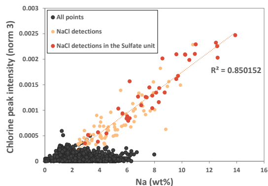
Fig. 1: Chlorine – Sodium correlation used to define halite detections (oxygen peak analysis not shown). Pure halite contains 39.3 wt% Na.
