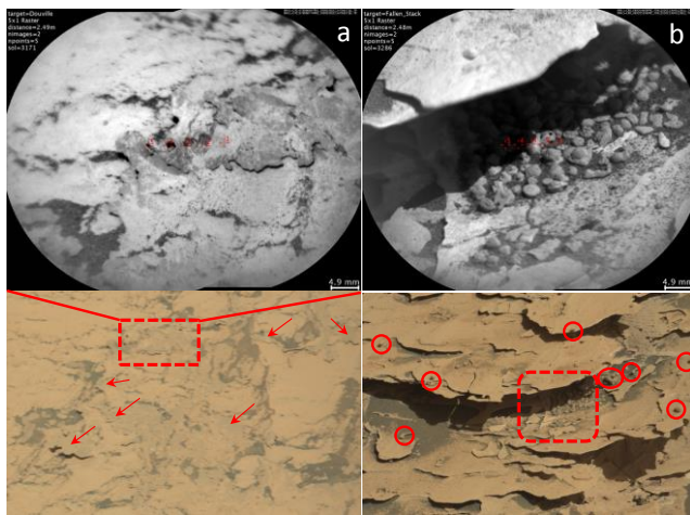
Fig. 3: Halite-rich features found in the Pontours member.
