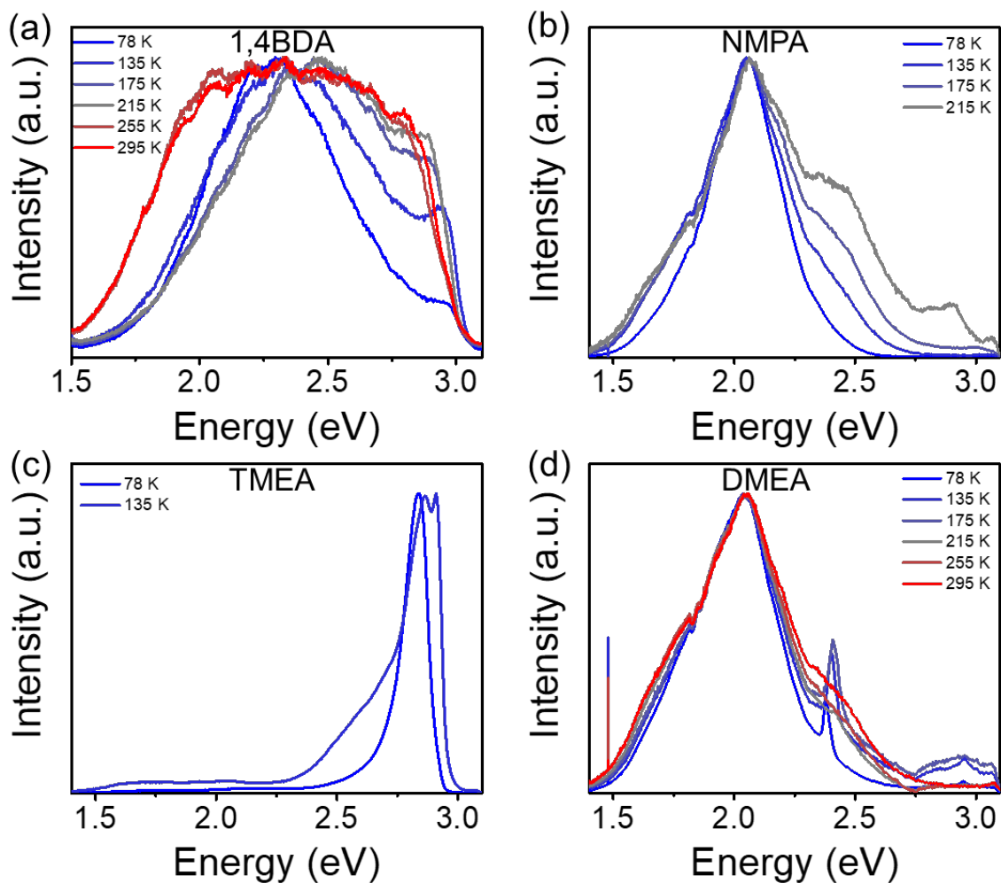
Figure 7. Normalized temperature-dependent PL spectra of (a) (1,4BDA) \text{Pb}_2\text{Br}_6 , (b) (NMPA) \text{Pb}_2\text{Br}_6 , (c) (TMEA) \text{Pb}_2\text{Br}_6 and (d) (DMEA) \text{Pb}_2\text{Br}_6 .
