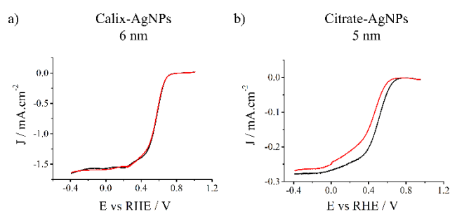
Fig. 3. Linear sweep voltammetry (LSV) curves recorded at 1600 rpm on a) 6 nm calix-AgNPs and b) 5 nm citrate-AgNPs before (black curves) and after (red curves) stability test in \text{O}_2 -saturated 0.1 M KOH solution. Normalized current density per electrochemically active surface area are reported.
