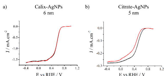
Fig. 3. Linear sweep voltammetry (LSV) curves recorded at 1600 rpm on a) 6 nm calix-AgNPs and b) 5 nm citrates AgNPs before (black curves) and after (red curves) stability test in \text{O}_2 -saturated 0.1 M KOH solution. Normalized current density per electrochemically active surface area are reported.
