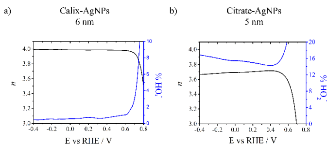
Fig. 2. Potential dependence of the number of electrons n (black lines) and the yield of \text{HO}_2^- (blue lines) produced during ORR experiments for a) 6 nm calix-AgNPs and b) 5 nm citrate-AgNPs.
