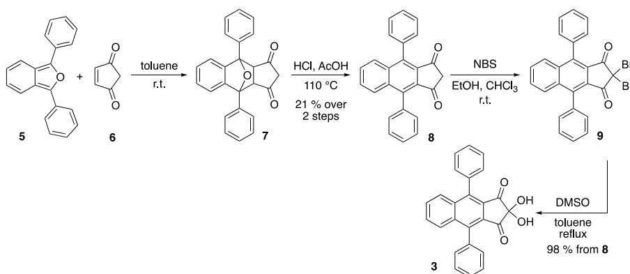
Scheme 1. Synthesis of Molecules 3 and 4
