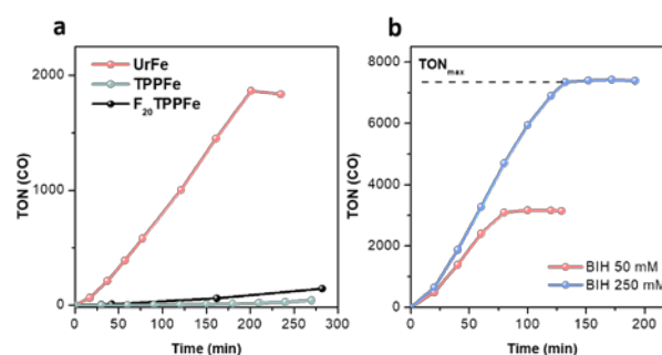
Figure 1 Time evolution of CO produced under a) visible light irradiation ( \lambda > 405 \text{ nm} , 100 W m -2 ) with TPPFe (green) F 20 TPPFe (black) or UrFe (red) as catalyst with 20 \mu\text{M} concentration; [Ru(bpy) 3 ] 2+ photosensitizer 1 mM, BIH sacrificial electron donor 50 mM in CO 2 -saturated DMF/H 2 O 9:1. b) light irradiation with a blue LED ( \lambda_{\text{em}} = 460 \text{ nm} , 100 W m -2 ) of UrFe as catalyst with 20 \mu\text{M} concentration; [Ru(bpy) 3 ] 2+ photosensitizer 1 mM, BIH sacrificial electron donor 50 mM (red) and 250 mM (blue) in CO 2 -saturated DMF/H 2 O 9:1.
