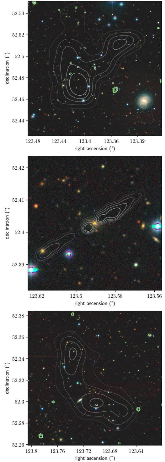
Fig. 3. Joint radio-optical views showing that the outer structures shown in Fig. 1 are best interpreted as a pair of RG lobes fed by central jets. On top of DESI Legacy Imaging Surveys DR9 ( g, r, z ) imagery, we show the LoTSS DR2 at various resolutions through contours at multiples of \sigma , where \sigma is the image noise at the relevant resolution. Top and bottom panels: translucent white 60'' contours at 3, 5, 7, 9, 11\sigma and solid light green 6'' contours at 4, 7, 10, 20, 40\sigma . Central panel: translucent white 6'' contours at 5, 10, 20, 40, 80\sigma .
