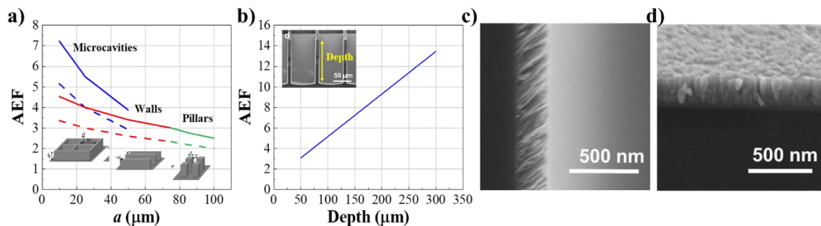
Figure 1. (a) Impact of cavity separation on AEF for different patterns. (b) Impact of depth on the AEF for the square microcavity. SEM cross-sectional images of the 3D photocatalyst (depth 150 μm) (b) inset, Si/ TiO 2 interface at (c) half-heights of the wall (d) bottom of the microcavities.
