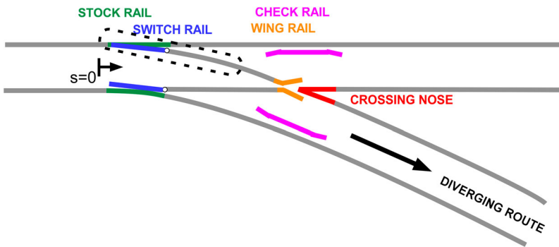
Figure 1. Turnout layout plan with diverging route in the facing traffic direction and rail body legends.
