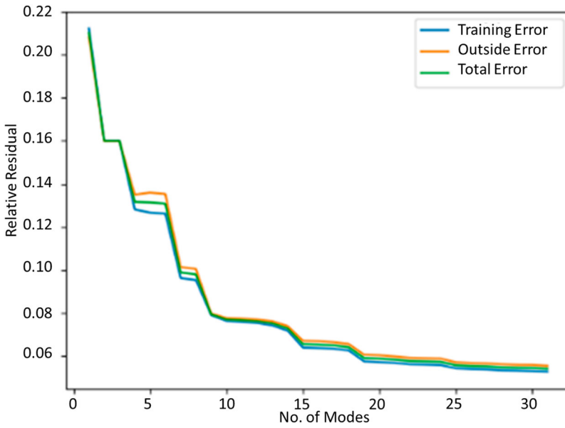
Figure 5. Convergence of the computational error. Relative residual r_p^N .
