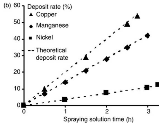
Figure 3. Deposit rate evolution versus spraying solution time, in case of iron based composite material (a) and copper-, manganese- and nickel-based composite materials (b).
