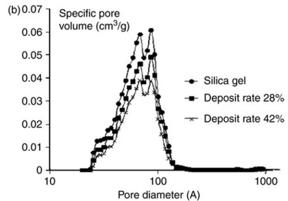
Figure 5. Pore size distribution for different metal loading in case of (a) iron composite materials on silica gel (b) manganese composite materials on silica gel.
