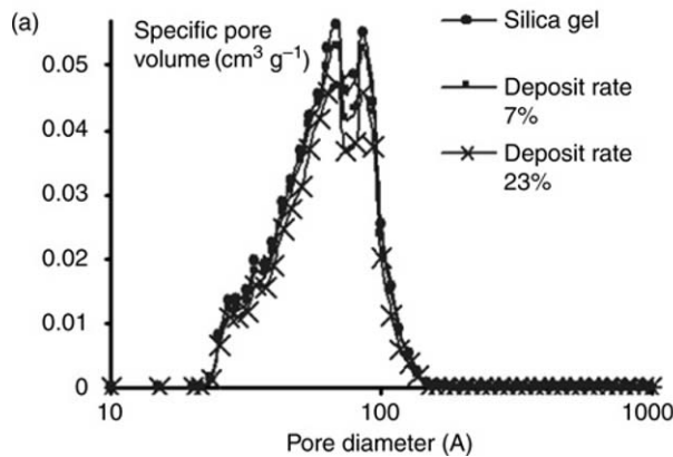
Figure 5. Pore size distribution for different metal loading in case of (a) iron composite materials on silica gel (b) manganese composite materials on silica gel.
