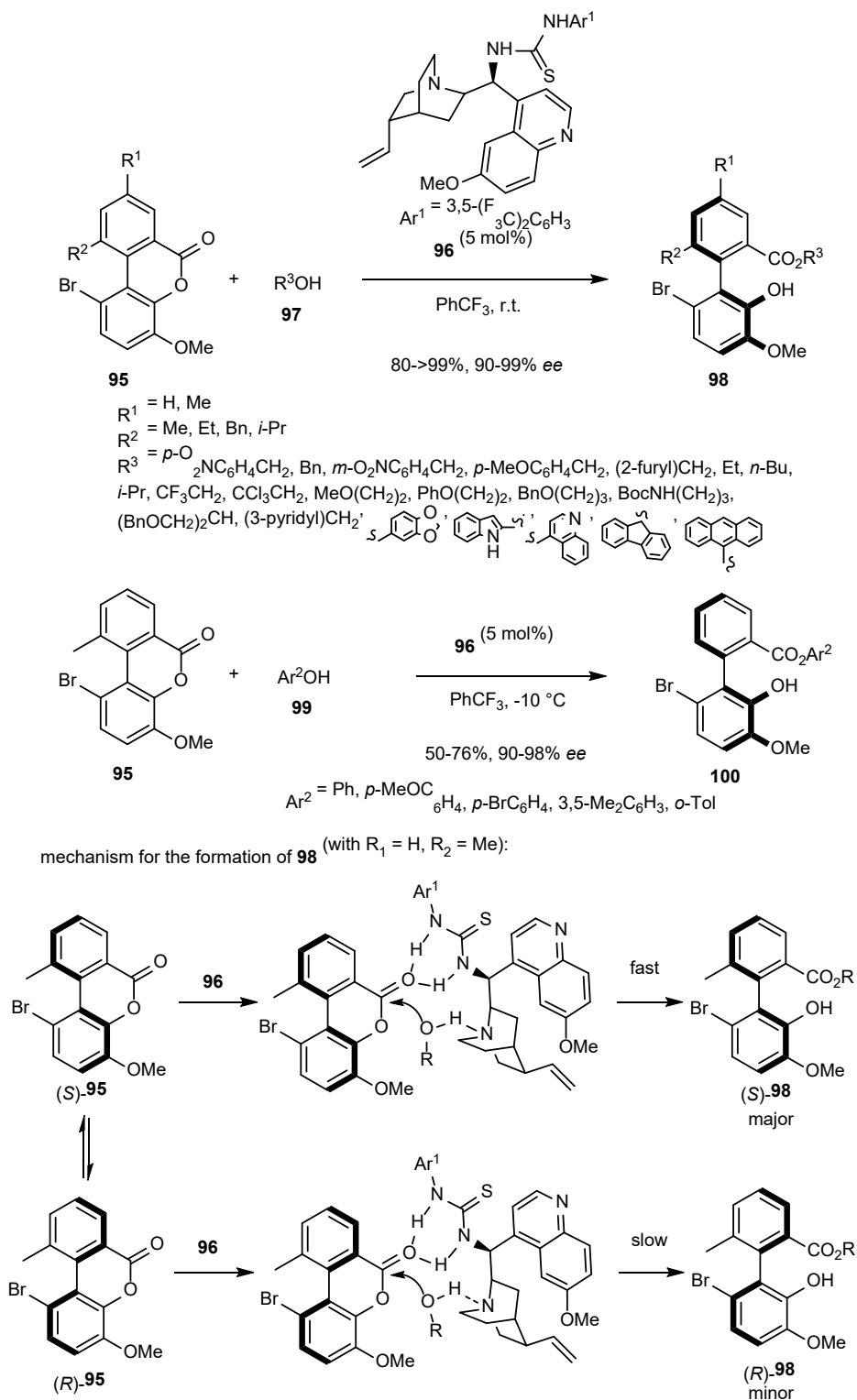
Scheme 20. Transesterifications of Bringmann's lactones.
