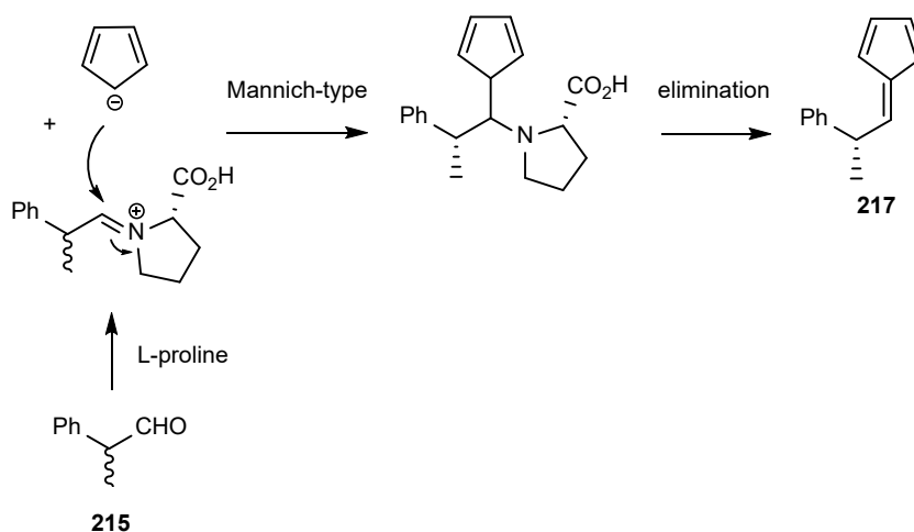
Scheme 46. Domino Mannich-type/dehydration reaction of 2-phenylpropanal with cyclopentadiene.
