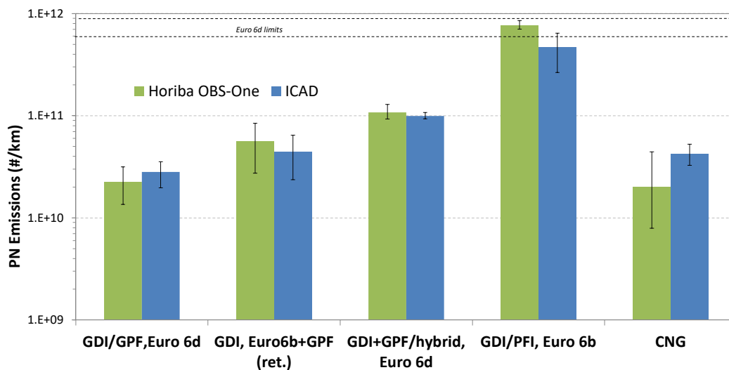
Figure 30. SUREAL-23 on-road tests for five vehicles. The ICAD measurements are compared to the commercially available Horiba OBS-1 system.
