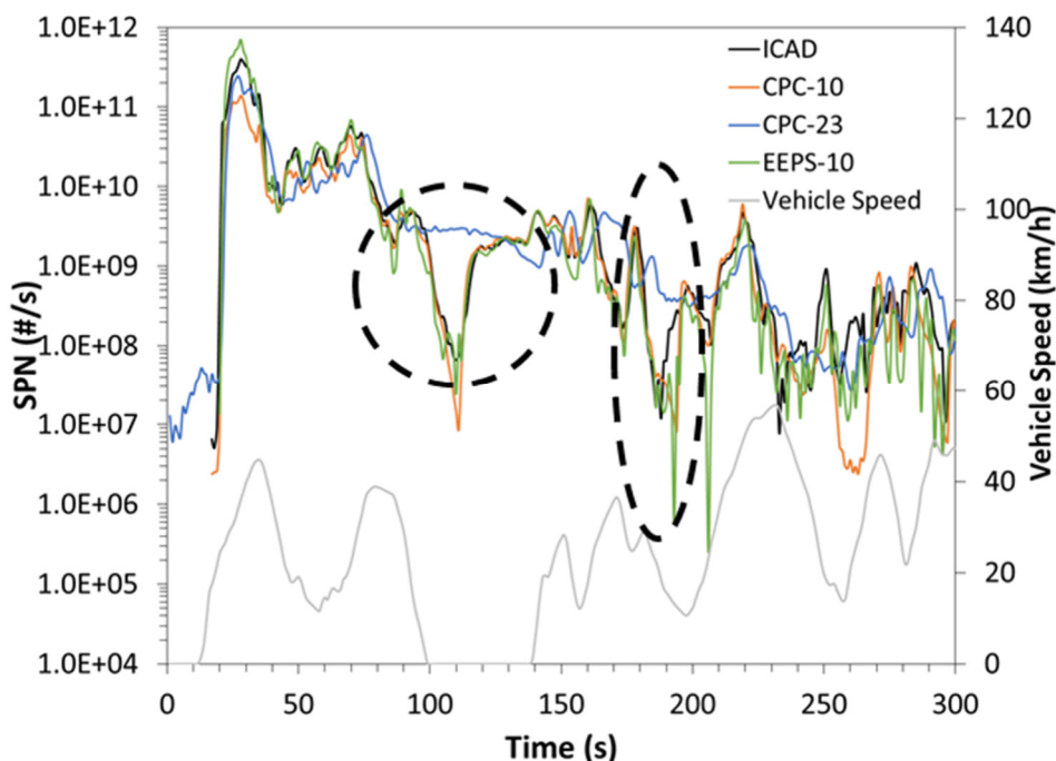
Figure 21. Multi-instrument measurement during the first 300 s of the WLTC. CPC-23 is connected to the PMP/CVS while all other instruments are connected to the tailpipe with the SUREAL-23 dilution system. EEPS=Engine Exhaust Particle Sizer.
