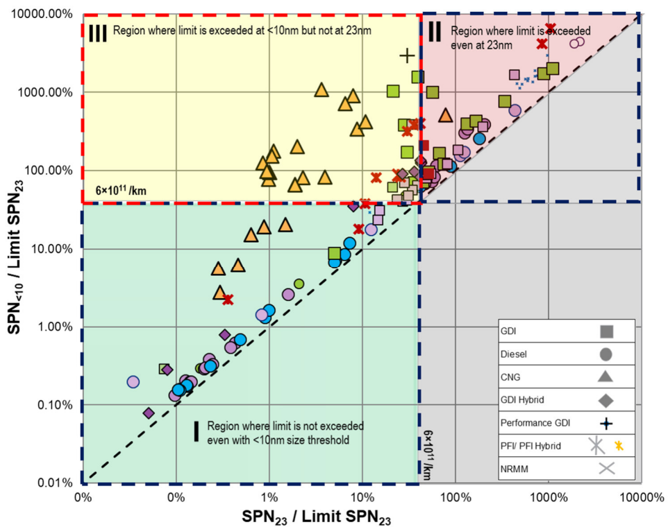
Figure 14. All Data gathered in DTT presented in the normalised form. Note: emission data are corrected for particle losses.
