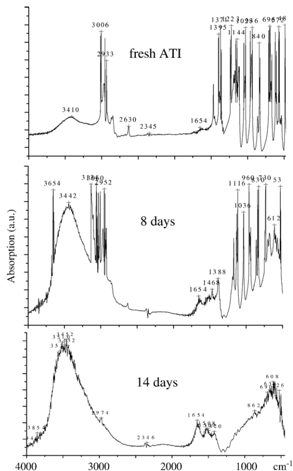
Fig. 3. Absorption FTIR spectra for ATI samples: fresh sample (top), and samples exposed to ambient atmosphere for 8 days (middle) and 2 weeks (bottom).
