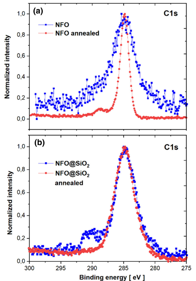
Fig. 12—Comparison between \text{C}1s states for as-received and annealed (a) NFO and (b) \text{NFO@SiO}_2 nanoparticles.
