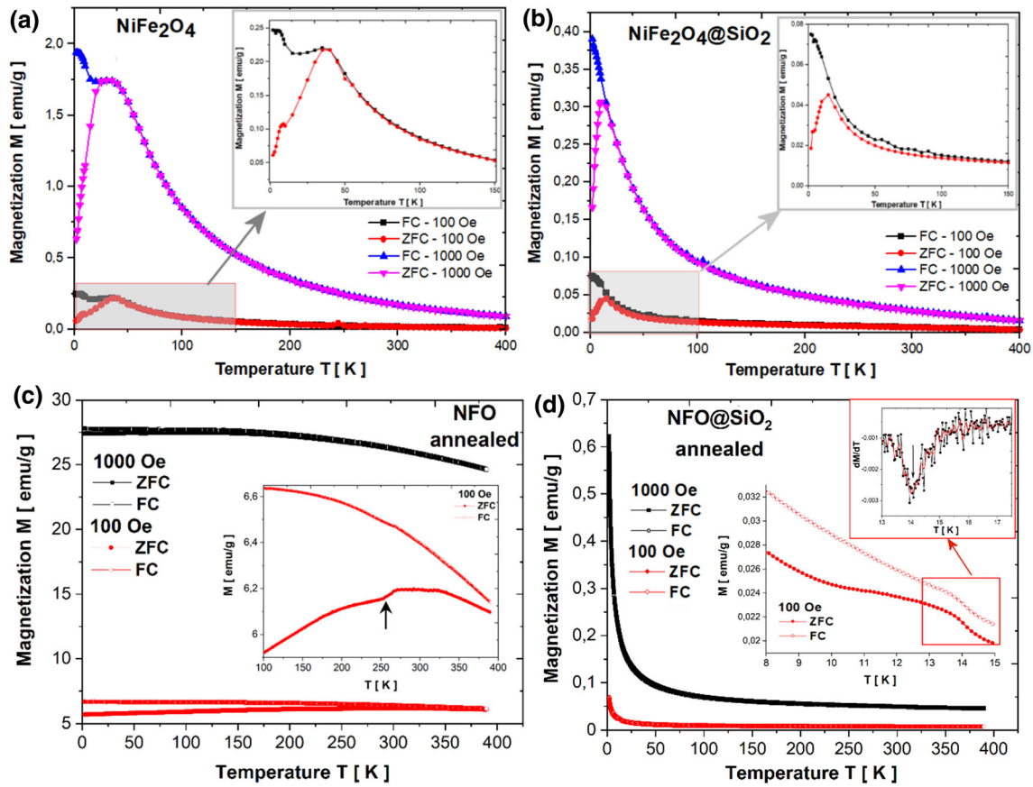
Fig. 7—Temperature dependences of DC magnetization measured at 100 Oe and 1000 Oe for as-received (a) and (b), as well as annealed (c) and (d), NFO and NFO@SiO 2 specimens, respectively.
