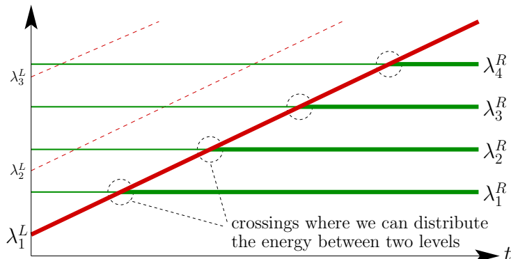
Figure 2: The behavior of the spectrum during our control process. The eigenvalues are split between two groups \lambda_j^L and \lambda_j^R . We deform the domain to ensure that the eigenvalue \lambda_1^L cross a suitable number of eigenvalues \lambda_j^R of the other group. At each crossing point, an accurate use of the tunneling effect enables to distribute the desired part of the energy carried by \lambda_1^L to \lambda_j^R .
