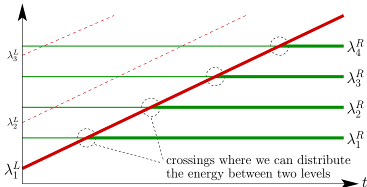
Figure 2: The behavior of the spectrum during our control process. The eigenvalues are split between two groups \lambda_j^L and \lambda_j^R . We deform the domain to ensure that the eigenvalue \lambda_1^L cross a suitable number of eigenvalues \lambda_j^R of the other group. At each crossing point, an accurate use of the tunneling effect enables to distribute the desired part of the energy carried by \lambda_1^L to \lambda_j^R .
