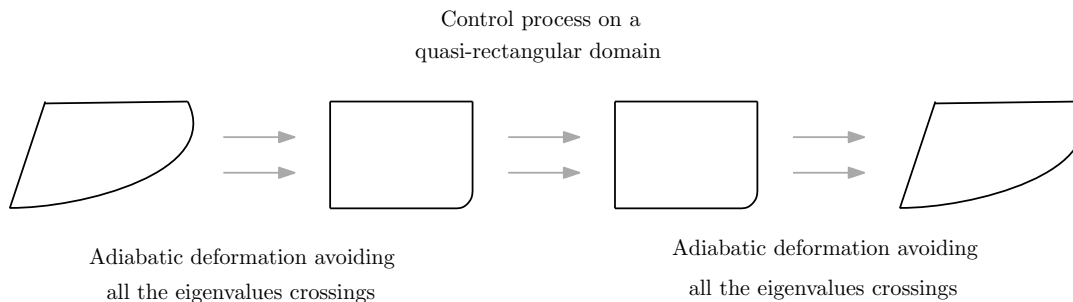
Figure 5: The figure shows how to use the tunneling effect to create superposed states. On the left, we pass adiabatically an eigenvalue crossing with a rectangular deformation and the quantum numbers of the state do not change thanks to Proposition 5.1. On the right, we break the symmetry and there is not any real crossing of eigenvalues anymore. Here, Corollary 5.4 yields that an adiabatic motion preserves the position in the spectrum and it switches the pure states. In the middle, we follow an interpolated deformation with the same speed, which produces an interpolated state. Physically, we use the tunneling effect to create a superposed state.
