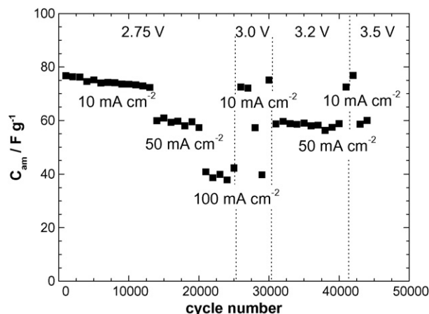
Fig. 4. Change of the specific capacitance of active material vs. cycles number for the CECA "Acticarbhone AB"/PYR 14 TFSI/CECA "Acticarbhone AB" supercapacitor from galvanostatic cycles at 10, 50, and 100 mA cm -2 for different cell cut-off at 60 °C.
