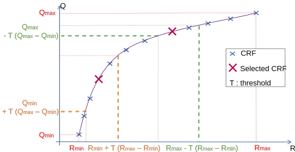
Fig. 1. Rate-quality optimized strategy to select CRF.
