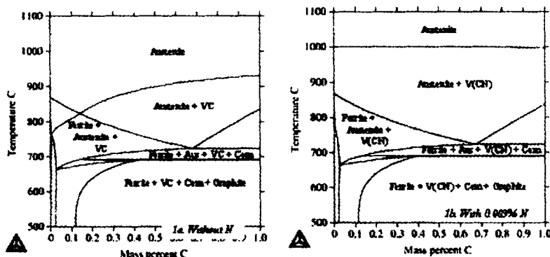
Fig. 1. Thermo-Calc Calculation Example: Isopleths for a HSLA steel, exploring how a small addition of nitrogen can change phase diagram and change the properties of material. Alloy content is Fe-1.5Mn-0.3Si-0.1V-C (in wt%). V(C,N) particles act as grain refiners
