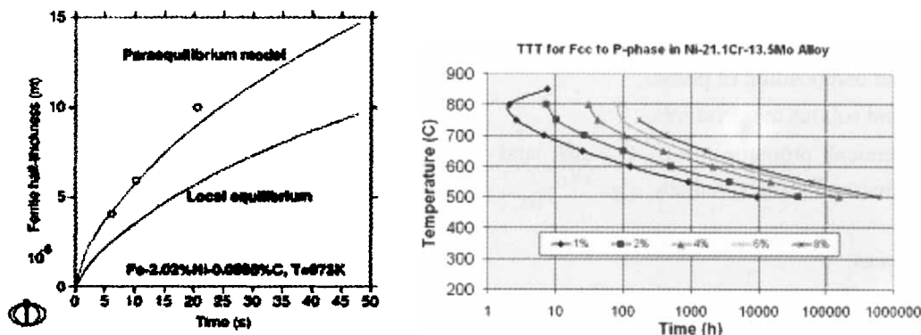
Fig. 5. DICTRA Simulation Example: Simulations of growth of ferrite into austenite in an Fe-2.02%Ni-0.0885% C alloy at 973 K (Result for local equilibrium at phase interface is compared with paraequilibrium assumption and recent experimental data), and of TTT diagram for FCC→P-phase transformation in an Ni-21.1%Cr-13.5%Mo alloy
