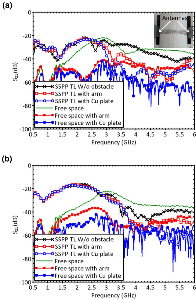
FIGURE 7 Measured transmission for the (a) even and (b) odd modes without (W/o) obstacles and for Spoof Surface Plasmon Polariton Transmission Line (SSPP TL) surrounding an arm or a copper plate positioned within a tunnel. In the inset, the experimental setup with curved SSPP TL with the antennas on each side
