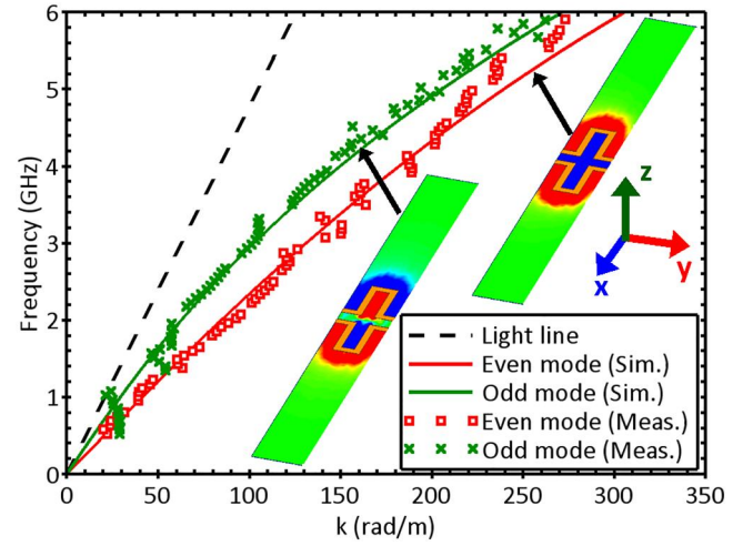
FIGURE 2 Simulated and experimental dispersion curves for the even and odd modes supported by the Spoof Surface Plasmon Polariton Transmission Line (SSPP TL). In the inset, z-component of the magnetic field simulated for the even and odd modes
