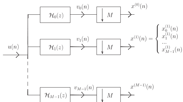
Fig. 1. Uniform filterbank with M subbands.
