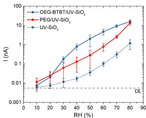
Figure 6. Absolute current curves as a function of RH for OEG-BTBT and PEG thin-film BC devices on UV-treated SiO 2 substrates (channel L = 5 μm). The electric response for the non-coated treated substrate is also reported. The dashed line indicates the experimental detection limit. Error bars correspond to the standard deviation acquired for n \geq 3 devices. Device channel length: L = 5 μm. RH range: 10–80%. Voltage bias applied: 2V.
