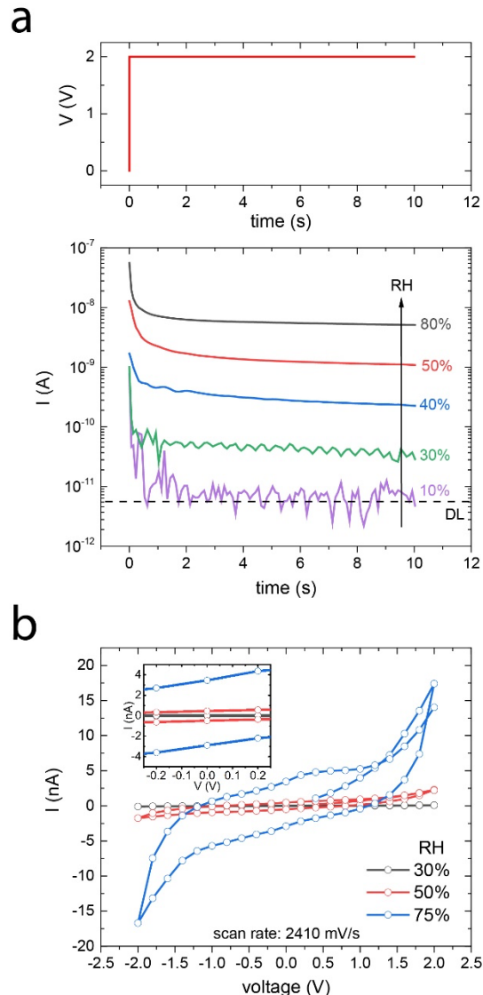
Figure 2. Electrical performance of RH-responsive chemiresistors (bottom-contact configuration). (a) Voltage bias stimulus (top) and respective chronoamperometric response of OEG-BTBT devices fabricated onto bare, non-treated SiO 2 at different RH levels (bottom). The current detection limit (DL) is indicated with a dashed black line. (b) I-V curves of OEG-BTBT onto bare SiO 2 measured at different RH at fast sweep rates (2410 mV/s). Inset: zoomed hysteric I-V response at small biases. Device channel length: L = 5 \mu\text{m} .
