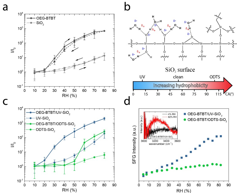
Figure 4. (a) Normalized current ( I/I_0 ) response as a function of RH for bottom-contact OEG-BTBT onto SiO 2 devices (solid line) and bare SiO 2 (dotted line) samples. The arrows illustrate the reversibility of the chemiresistor response upon the RH increase and following decrease. Dashed and dash-dotted lines indicate values obtained while decreasing the RH (see arrows direction). (b) H-bond interactions of water molecules with silanol and Si–O–Si groups of the SiO 2 surface. (c) Current response of OEG-BTBT devices fabricated on treated SiO 2 (UV/ozone and ODTS, solid lines) and bare substrates (dotted lines). For OEG-BTBT/ODTS-SiO 2 and ODTS-SiO 2 devices, the current reaches the instrumental DL at RH ≤ 40%. (d) Sum frequency generation (SFG) integrated intensity of the 3300 cm -1 O–H stretching band of 50-nm OEG-BTBT thin films on UV-SiO 2 and ODTS-SiO 2 substrates. Inset: SFG spectrum of the OEG-BTBT/UV-SiO 2 interface at low (4%) and high (82%) RH. Current values and error bars in (a) and (c) correspond to the average
