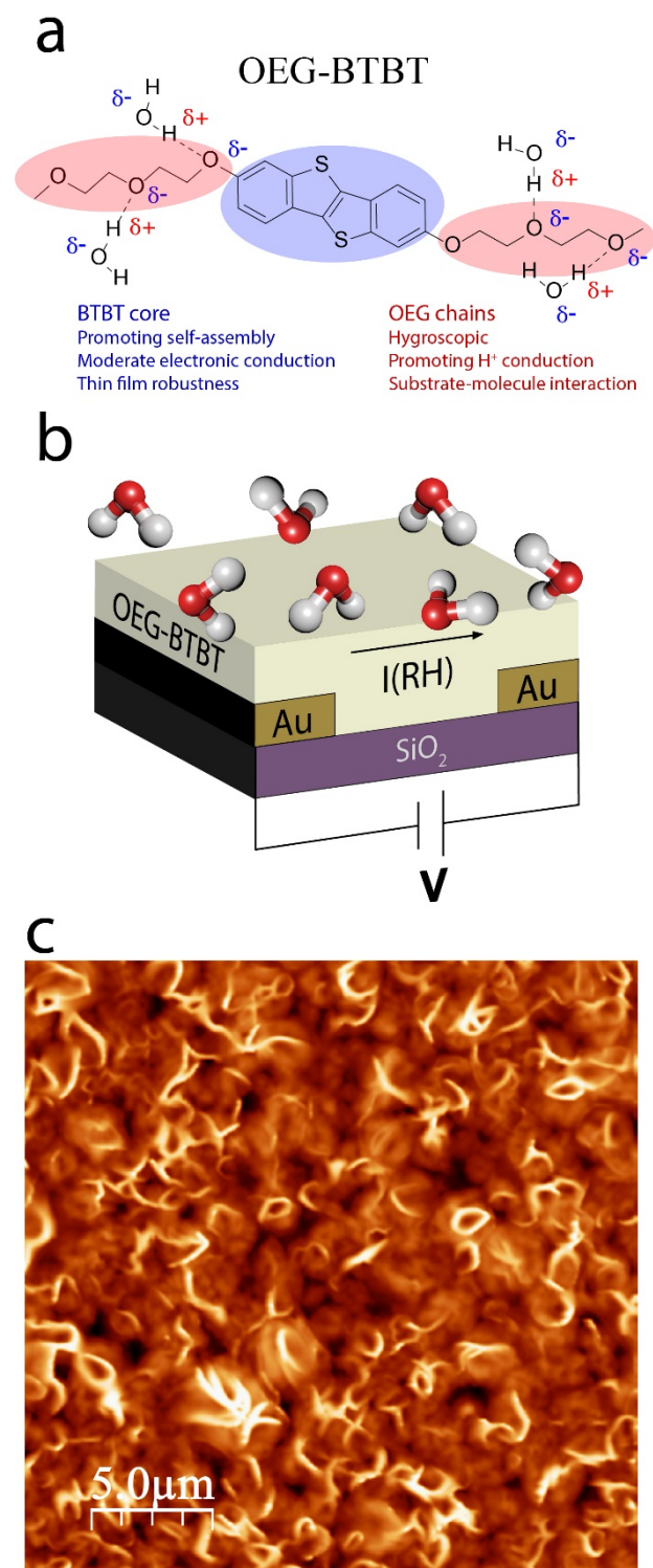
Figure 1. (a) Chemical structure of OEG-BTBT molecule and its interaction with atmospheric water molecules via H-bonding interactions. (b) Sketch of the OEG-BTBT humidity-responsive chemiresistor. The RH-sensitive device current I(RH) is recorded upon application of a constant DC bias ( V ). (c) AFM height image of the spin-cast OEG-BTBT film surface deposited on SiO 2 . Z-scale: 380 nm, R RMS : 67 nm.
