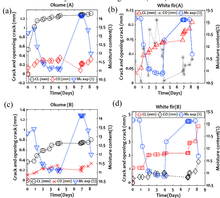
Fig. 6. Impact of moisture content variations on crack openings (a) Okume test 1; (b) White fir test 1; (c) Okume test2; (d) White fir test 2.
