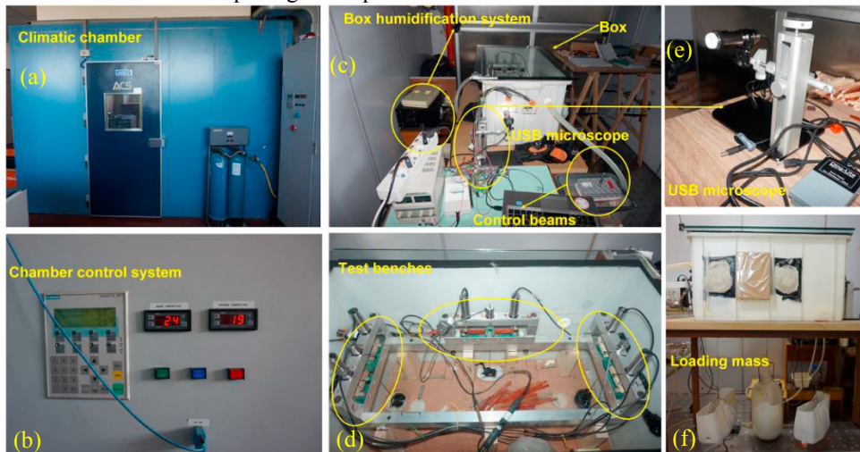
Fig. 2. (a) Climatic chamber; (b) chamber control system; (c) experiment set up ;(d) test benches; (e) USB microscope ;(f) loading for creep test.
