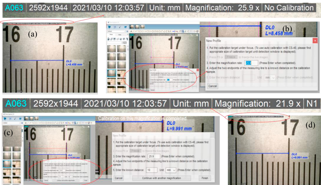
Fig. 3. Estimation of cracking parameters with the USB microscope (a) image without calibration; (b) calibration of magnification; (c) calibration of real distance; (d) calibrated image.
