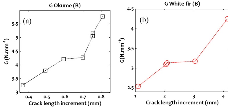
Fig. 7. Energy restitution rate for test 2 (a) Okume; (b) White fir
