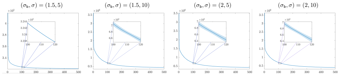
Fig. 3: Decay of the objective value along 500 iterations for Westconcord example, using different combinations of (\sigma_b, \sigma) . We considered 10 random sampling for p^0 and \beta^0 . The continuous line in the plot represents the mean objective value at each iteration and the shaded area, highlighted in the zoomed region at the centre of the plot spanning over 20 iterations, corresponds to the confidence interval related to the standard deviation.
