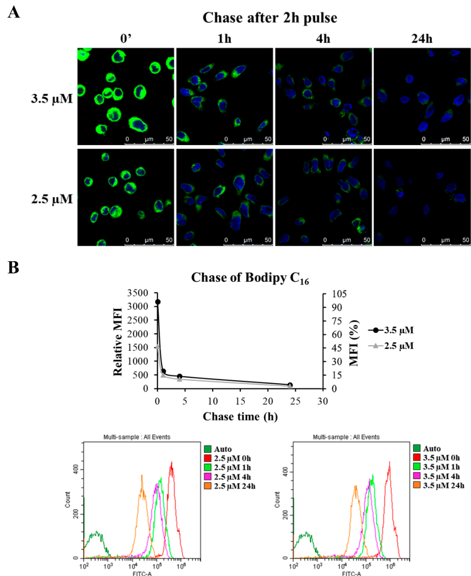
Figure 10. Chase of Bodipy C 16 after 2h pulse. 0.3 \times 10^6 GEN2.2 cells were pulsed for 2 h with 2.5 μM or 3.5 μM of Bodipy C 16 in complete medium supplemented with 0.3% FBS. Afterwards, cells were washed and chased in complete medium containing 10% FBS according to the times reported in the figure. (A) For confocal microscopy analysis, cells were placed on a microscope slide and fixed in PFA 4%. To visualize nuclei (blue), GEN2.2 cells were stained with DAPI. Images were acquired with the confocal microscope Leica TCS SP5 and processed with the software LAS AF version 1.6.3 (Leica Microsystems). Objective 63.0X. DIC: Differential Interference Contrast. Scale bars 0–50 μm. (B) Cell fluorescence was analysed by FC and reported as relative MFI and percentage of MFI (upper panel). The corresponding flow cytometry plots were reported in the lower panel. A representative experiment, out of three independent experiments that yielded similar results, is shown.
