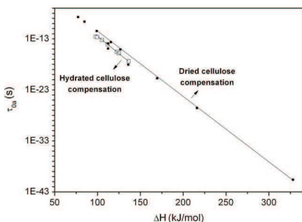
5. Pre-exponential factor of \alpha mode of hydrated and dried cellulose as a function of activation enthalpy.
