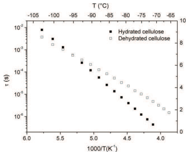
Fig. 2. Arrhenius diagram for hydrated (pristine) and dried cellulose for the low temperature ( \gamma ) relaxation mode.
