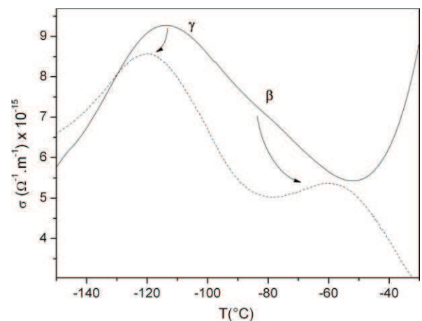
Fig. 5. Complex TSC thermograms of hydrated (solid line) and dried cellulose (dashed line) for the low temperature \gamma and \beta relaxation modes.
