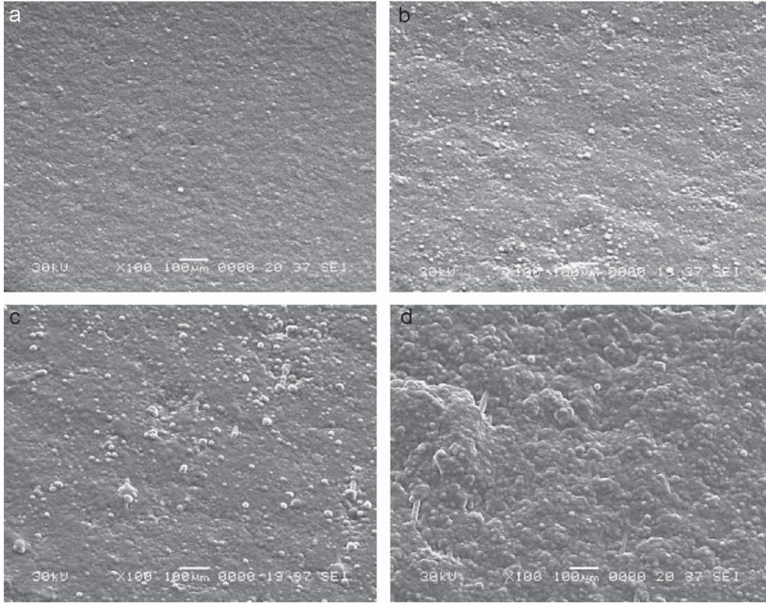
Fig. 3. (a) SEM image of parylene deposition (10 \mu m/100% activated carbon) (100). (b) SEM image of parylene deposition (10 \mu m/70–30% activated carbon-CNTs) (100). (c) SEM image of parylene deposition (10 \mu m/50–50% activated carbon-CNTs) (100). (d) SEM image of parylene deposition (10 \mu m/100% CNTs) (100).
