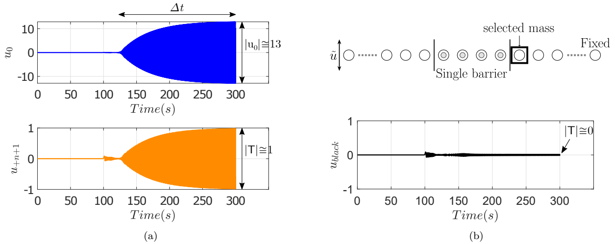
Figure 12: (a) Oscillations in time of displacements u_0 and u_{+n+1} of the masses evidenced respectively in blue and orange in figure 10. (b) Oscillation in time of the displacement of the first cell after a barrier without defect (sketch above). Material parameters: \theta = 1 , \varepsilon = 1 , m_2 = 0.01 Kg, k_2 = 1 N m -1 .
