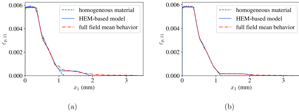
Fig. 9. Comparison between the mean plastic strain of the HEM-based model and the mean plastic strain of the full field reference solution for d_{in} = 0.2 . (a) Test case 1 (a) and (b) Test case 5.
