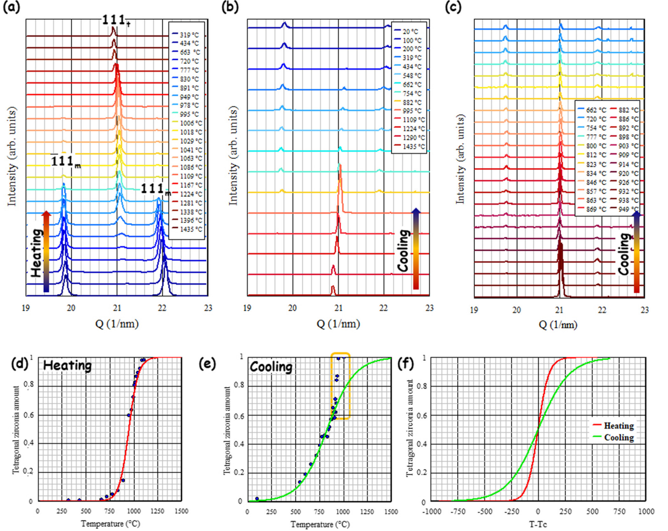
FIG. 2. Volume fraction of tetragonal zirconia as a function of temperature during heating and cooling. (a)–(c) Part of the XRD patterns recorded during the heating and cooling processes. During cooling, the diffraction patterns were recorded roughly every 6°C [see (c)]. (d),(e) Fit with a sigmoidal law of the evolutions of the volume fraction of tetragonal zirconia as a function of temperature during heating and cooling. (f) Evolution of the tetragonal volume fraction with respect to the critical m \rightarrow t and t \rightarrow m phase transition temperatures. Only the crystal size effect is considered in (f).
