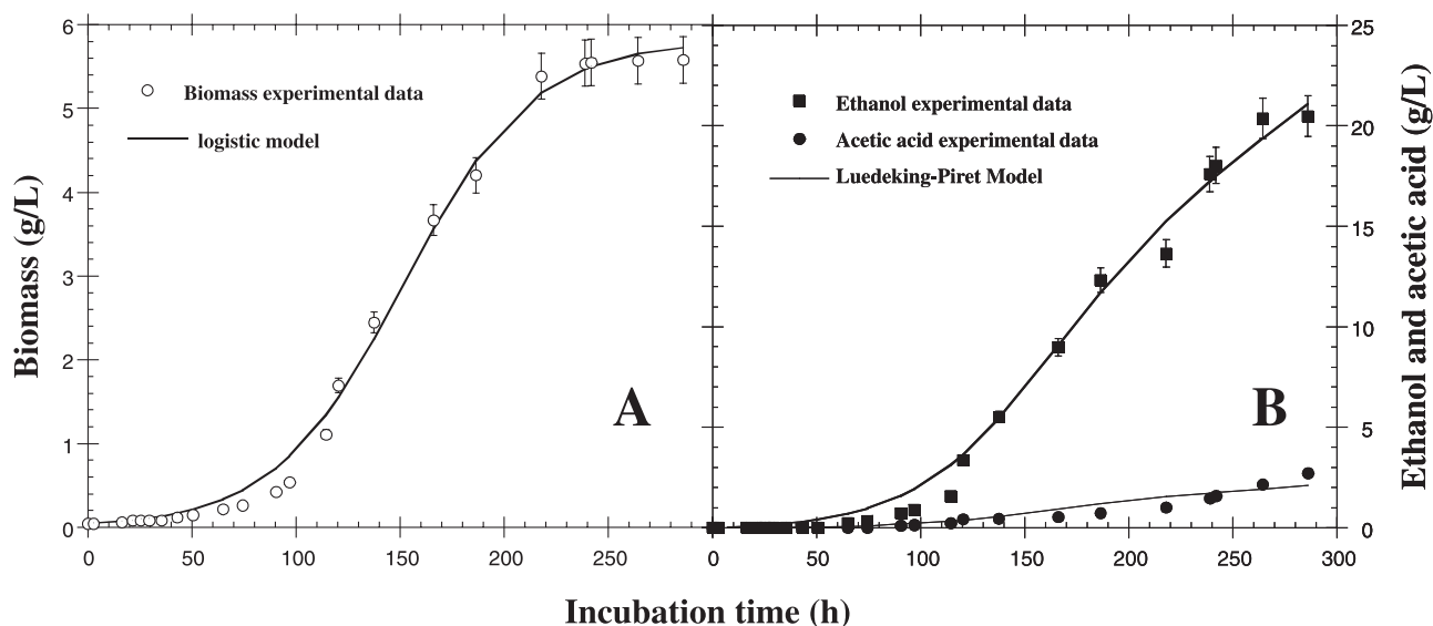
Fig. 5. Representation of biomass concentration by the logistic model at 15 °C (A) and representation of ethanol and acetic acid concentration by the Luedeking–Piret Model (B).
