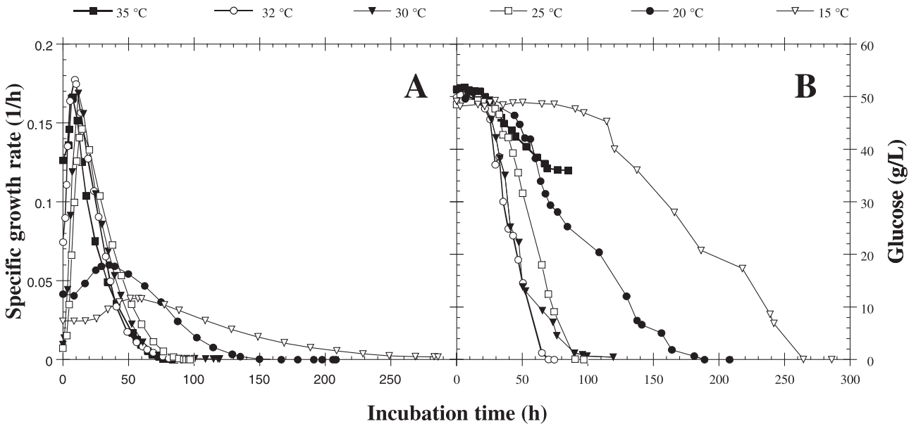
Fig. 2. Temperature influence on specific growth rate (A) and glucose consumption (B) during fermentation.
