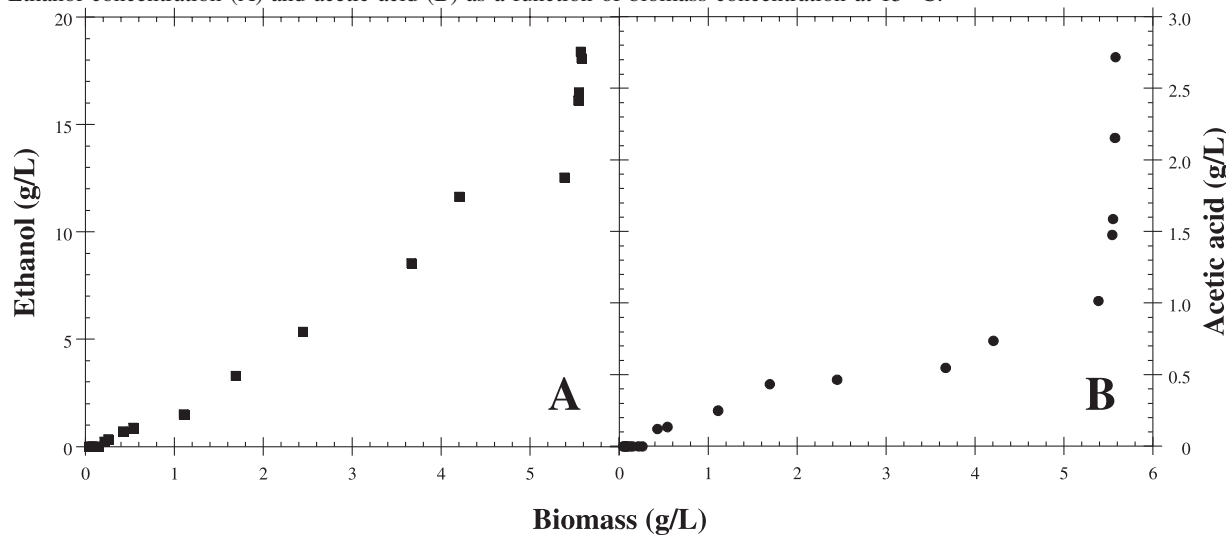
Fig. 6. Ethanol concentration (A) and acetic acid (B) as a function of biomass concentration at 15 °C.
