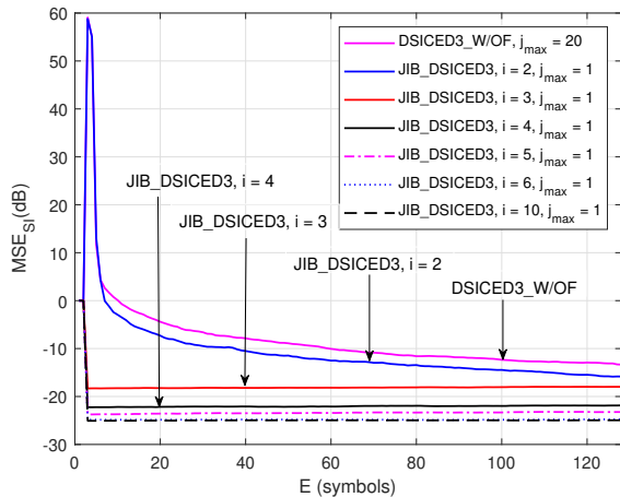
FIGURE 3. MSE_{S1} (dB) after the i -th decoding iteration versus E symbols; p_{SI}/\sigma_w^2 = 30 dB and p_B/\sigma_w^2 = 20 dB.
