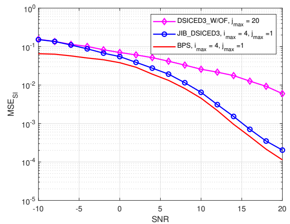
FIGURE 5. MSE_{S1} versus the SNR, p_B/\sigma_w^2 ; p_{SI}/\sigma_w^2 = 30 dB and E = 128 symbols.
