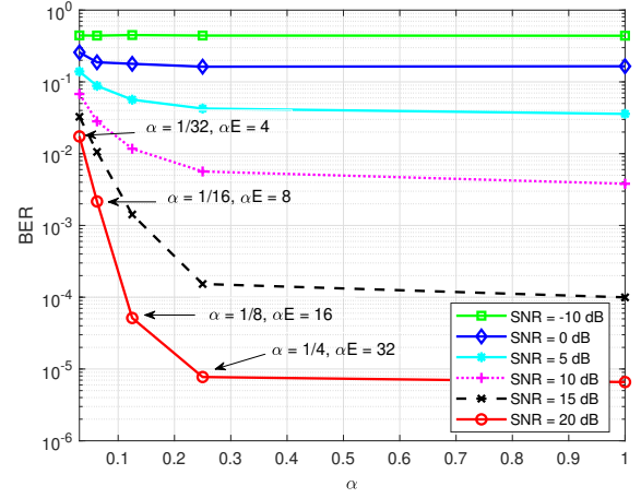
FIGURE 12. BER of JIB_DSICED3_PF scheme versus \alpha ; i_{max} = 4, j_{max} = 1, p_{SI}/\sigma_w^2 = 30 dB and E = 128 symbols.
