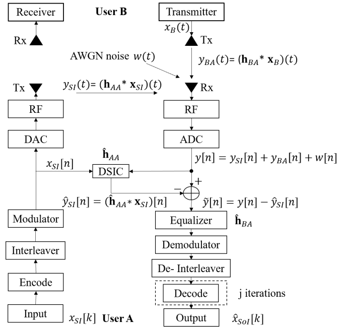
FIGURE 1. SISO FD transmission with DSICED3_W/OF process.
