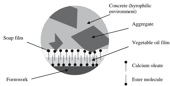
Fig. 19 Organisation of a soap film at the concrete/formwork interface
