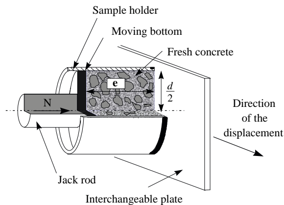
Fig. 4 Tribometer principle
