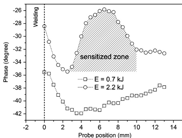
Fig. 9. Comparison of the impedance phase measured at 0.5 Hz with the distance from the weld string.
